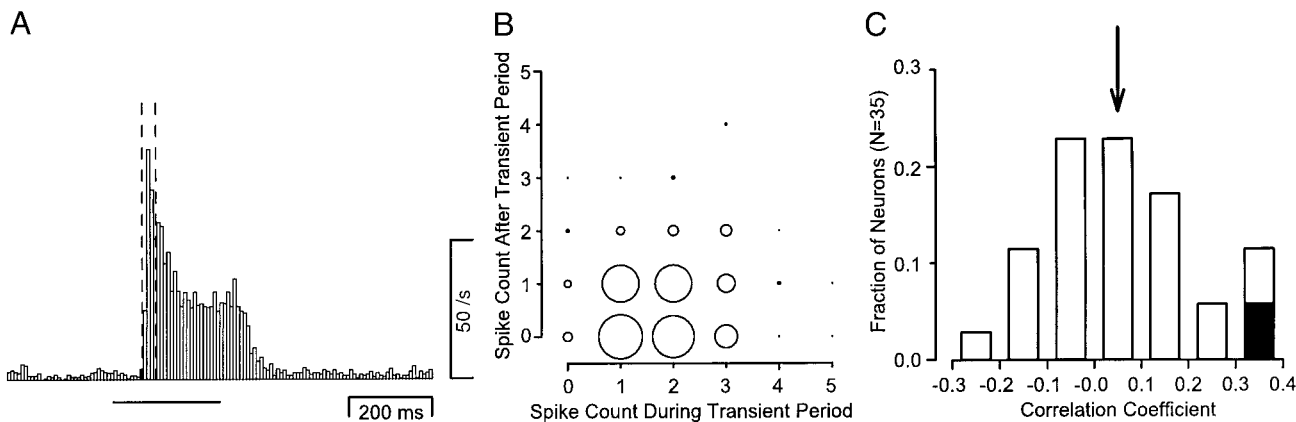
FIG. 10. The effect of spiking activity during the transient period on subsequent firing. A: histogram showing the response of an MT neuron to a step of target speed accumulated in 8-ms wide bins from 265 repetitions of the preferred stimulus for the neuron under study. The 2 vertical dashed lines indicate the period defined from the average response as the transient period. The transient period is not aligned with the bins of the histogram because it was determined from separate analysis on a 1-ms time scale. B: the size of each circle summarizes the number of individual trials in which the number of spikes during transient interval and the subsequent 16 ms had the values indicated by the location of the circle on the x and y axes. The largest circle indicates a combination of transient and sustained spike counts that occurred in 45 different trials. C: the distribution of correlation coefficients from plots like that in B for the 37 neurons in our sample population. Filled and open bars indicate correlation coefficients that were or were not statistically significant ( t -test, P > 0.05 ). The downward arrow above the histogram indicates the mean correlation coefficient in our sample, which was 0.05.
