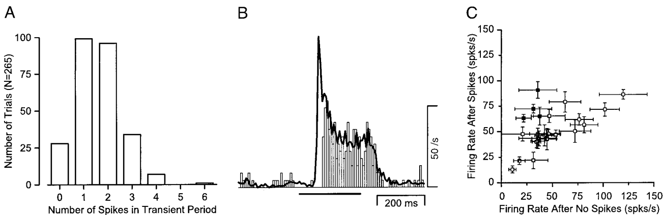
FIG. 11. Comparison of time course of response in trials with and without spikes in the transient period defined from the average response. A: the frequency of different spike counts during the transient period for the same example neuron used to construct the histogram in Fig. 10A. B: the histogram shows the firing rate of the neuron for 26 trials that lacked spikes during the transient period defined from the average response. The thick trace shows the average response of the neuron for 239 trials in which 1 or more spikes occurred during the transient period. C: graph showing the effect of spiking during the transient interval on the adaptation of MT neurons. Each point plots data from 1 neuron. The y axis plots firing rate during the 16 ms after the transient interval when 1 or more spikes occurred in the transient interval. The x axis plots firing rate during the 16 ms after the transient interval when no spikes occurred in the transient interval defined from the average firing rate. Filled symbols indicate 4 neurons that showed statistically different responses under these 2 conditions, depending on the presence of spiking in the transient period. Horizontal and vertical error bars show the standard errors of the mean for the conditions of spiking or no spiking during the transient period.
