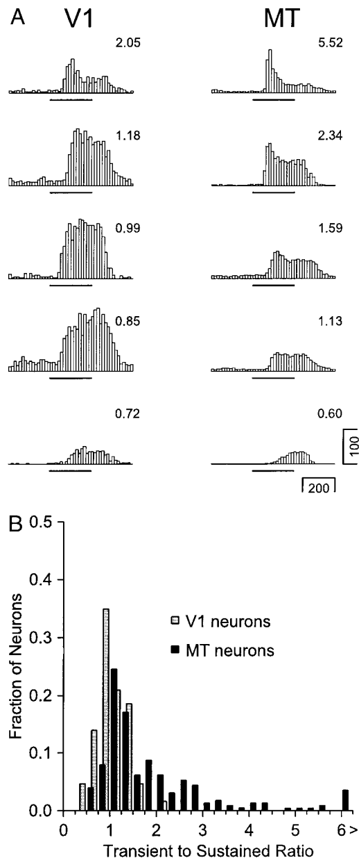
FIG. 9. Absence of transient responses in V1 neurons. A : examples of the spectrum of transient responses of V1 and MT neurons to steps of texture speed. — (below each histogram), the timing and duration of texture motion of the preferred direction and speed of the neuron being recorded. The number at the top right of each histogram indicates the transient-sustained ratio. B : quantitative comparison of the distribution of transient-sustained ratios in V1 and MT neurons. ■ and □, summary of our samples of 213 neurons in MT and 63 direction-selective neurons in V1, respectively.
