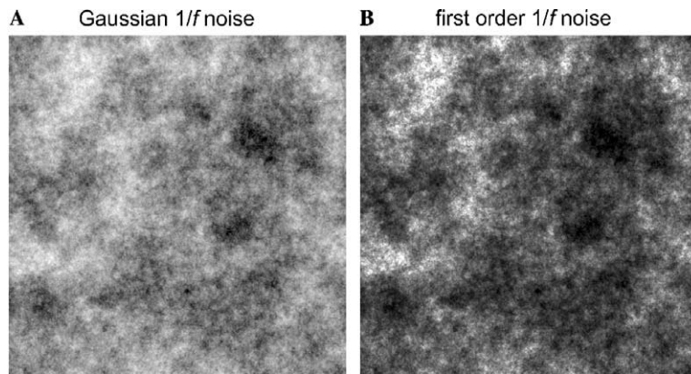
Fig. 11. Samples of 1/f noise. (A) Standard 1/f noise, which has a Gaussian pixel luminance distribution. In this noise there is a large negative correlation between local luminance and contrast. (B) First-order 1/f noise, which has the average pixel luminance distribution of natural (rural) images. In this noise there is a weak negative correlation between local luminance and contrast.
