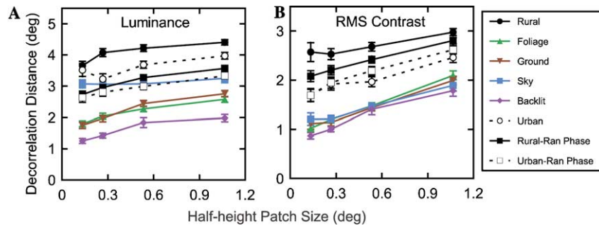
Fig. 7. Distance between image patches where the correlation drops on average to a value of 0.25, as a function of image patch size. (A) The correlations between the luminances of the image patches. (B) The correlations between the RMS contrasts of the image patches.
