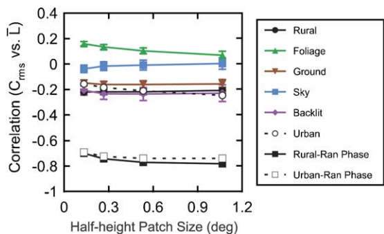
Fig. 6. Correlation between local luminance and local RMS contrast as a function of analysis patch size. The black and open squares show the correlations for images where the spatial phases have been randomized; a correlation of approximately -0.8 is also obtained for 1/f noise.
