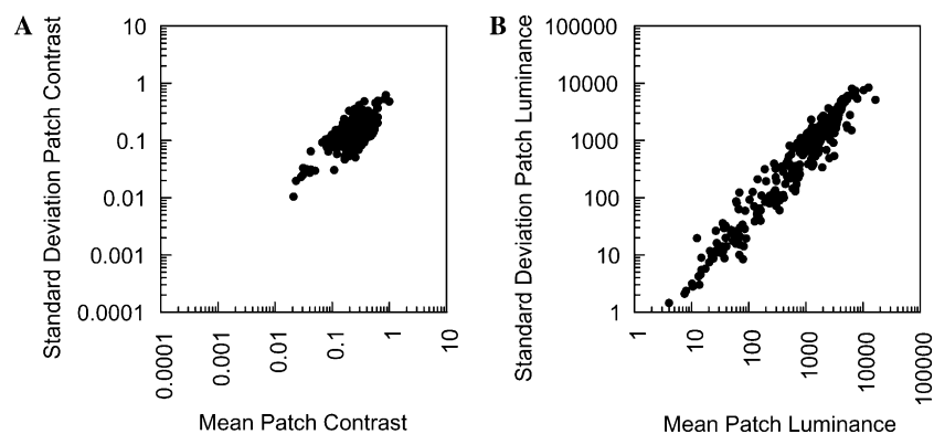
Fig. 9. Distributions of local contrast and local luminance for each of the 300 rural images. Each data point represents a distribution (a mean and a standard deviation) for a particular rural image. (A) Scatter plot of the mean local rms contrast and the standard deviation of local rms contrast. (B) Scatter plot of the mean local luminance and the standard deviation of local luminance. Note that all axes were set to be equal in numbers of log units. The analysis patch diameter was 0.54 deg.
