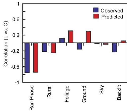
Fig. 10. Predicted effect of the first-order statistics (the pixel luminance distributions) on the correlation between local luminance and contrast. Natural images where the phase is randomized have a pixel luminance distribution that is symmetric about the mean (i.e., approximately Gaussian). In this case, the predicted correlation is highly negative (nearly -0.8 ). The skewed pixel luminance distributions of natural images shift the correlations near to or above zero. The parameters describing the pixel luminance distributions are as follows (the last number is the percentage of variance accounted for; see text for equations): ran phase ( a = 74 , b = 1719 , n = 0.66 , 99.1%), rural ( a = 1.28 , b = 2.04 , n = 0.41 , 99.4%), foliage ( a = 0.91 , b = 0.65 , n = 0.86 , 99.8%), ground ( a = 1.0 , b = 0.86 , n = 0.87 , 99.7%), sky ( a = 1.12 , b = 1.16 , n = 0.98 , 98.2%), and backlit ( a = 1.05 , b = 0.82 , n = 0.5 , 98.9%).
